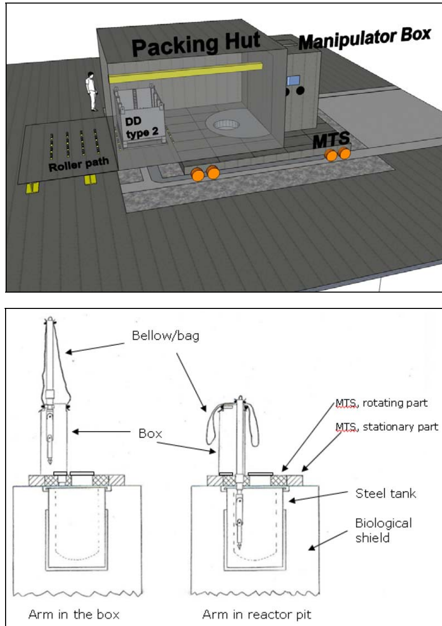
Figure 5. Model of intended setup of Moveable Top Shield (MTS), manipulator box and packing hut on top of DR 3. The lower section of the figure shows the suggested operation of the robotic tool arm.
